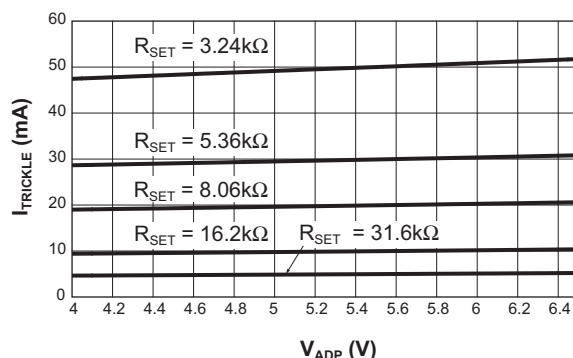
Preconditioning Charge Current vs. Supply Voltage
